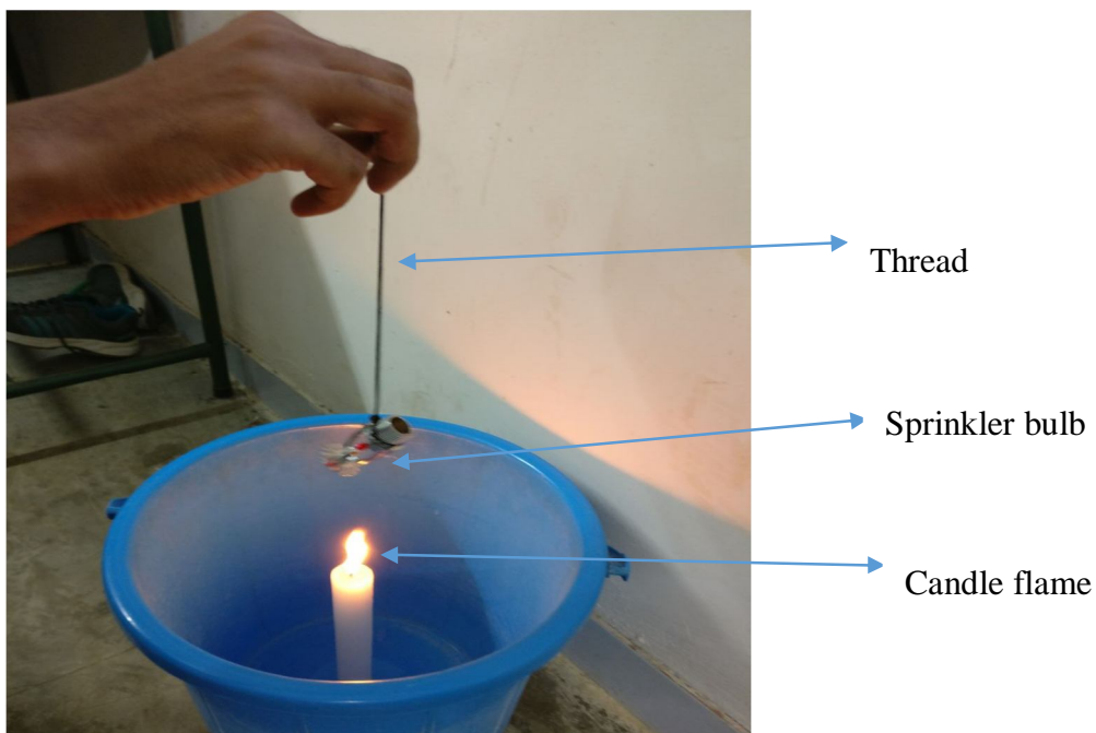
Fig 4.20 Experimental setup
