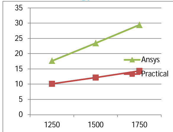
Graph No.02 pressure vs. deflection result for FEA analysis
