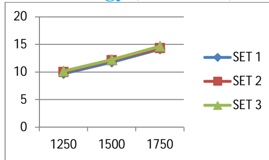
Graph No.01 pressure vs. deflection for Practical analysis results
