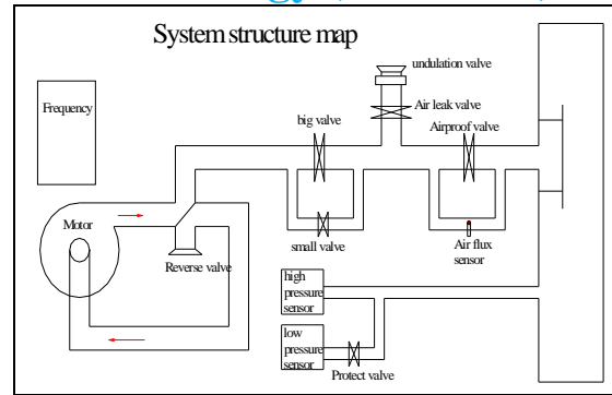
Fig.01 Practical Setup of WTM
