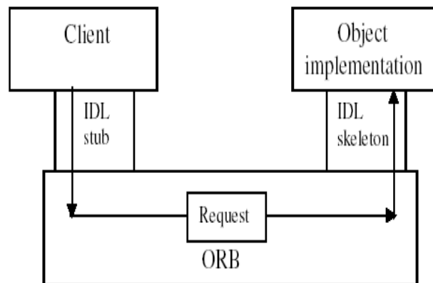
Figure 3.3: Remote method invocation when client and server are using the same ORB.
