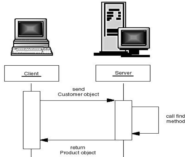
Figure 2: RMI using Client & Server Object
