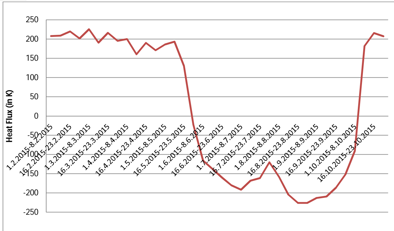
Fig 17: Time series plot of heat flux of 2015 for Station BHUBANESWAR (Lat.- 20.25 °N,Long.-85.8333 °E)
