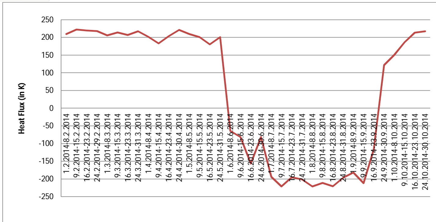
Fig 19: Time series plot of heat flux of 2014 for Station:CALCUTTA (Lat.- 22.65 °N,Long.-88.45 °E)
