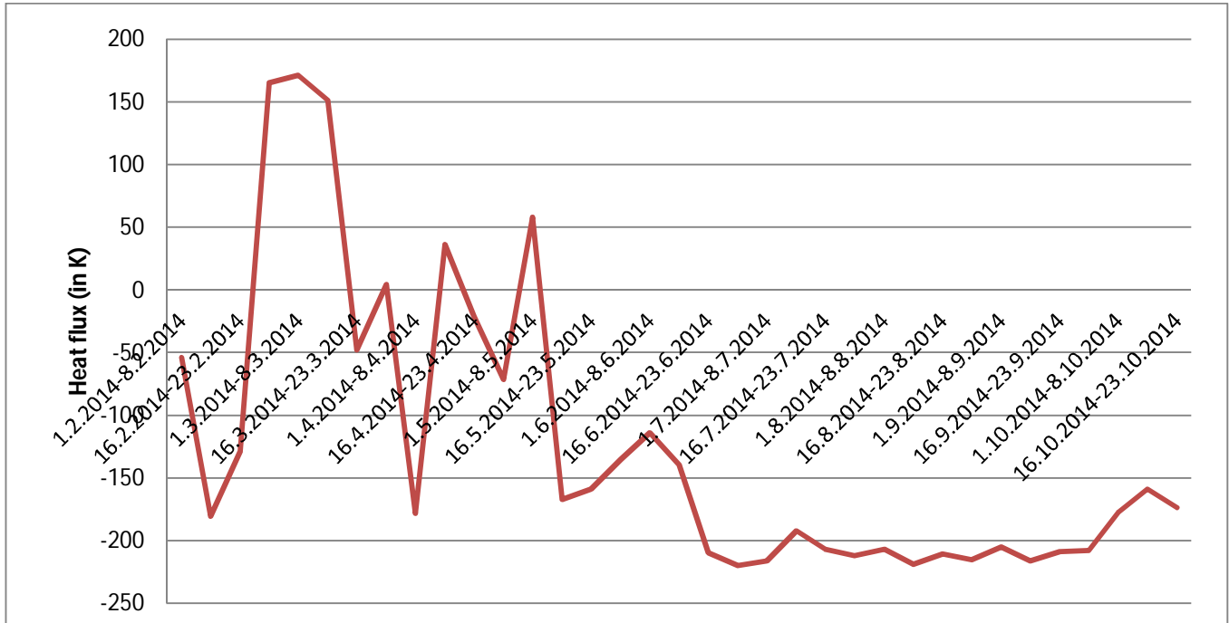
Fig 7: Time series plot of heat flux of 2014 of Station TRIVANDRUM (Lat.- 8.4833 °N,Long.-76.95 °E)
