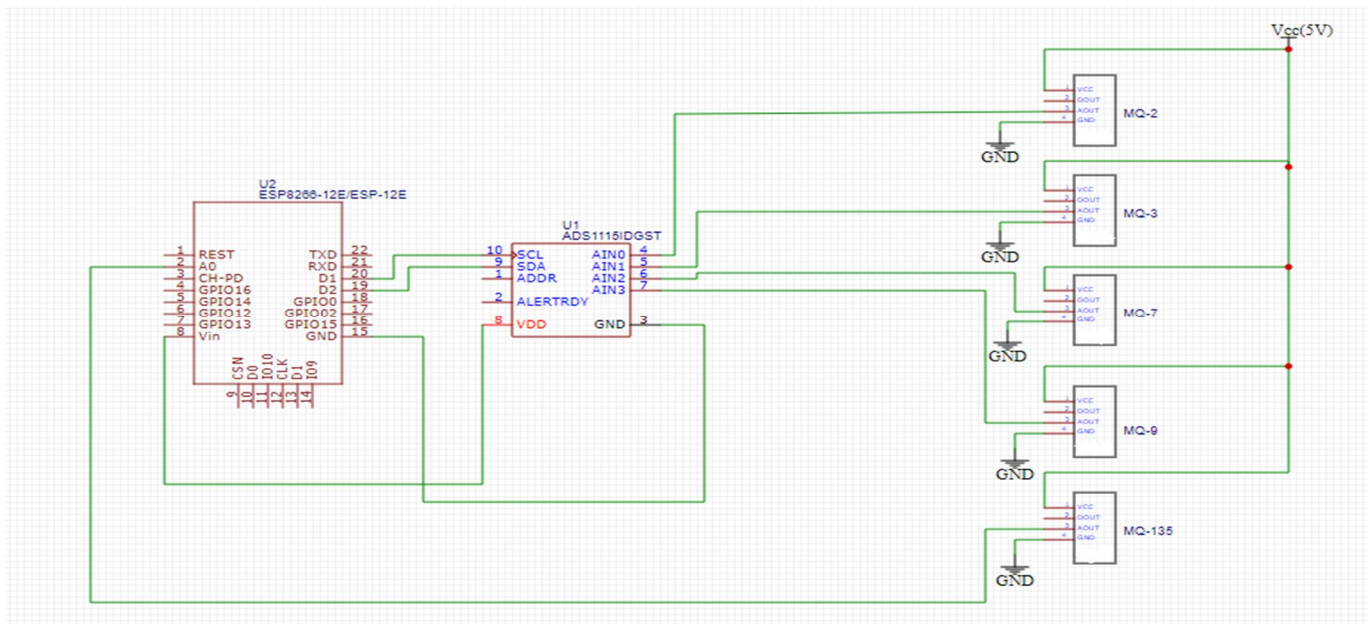
Fig. 2 System Schematic
