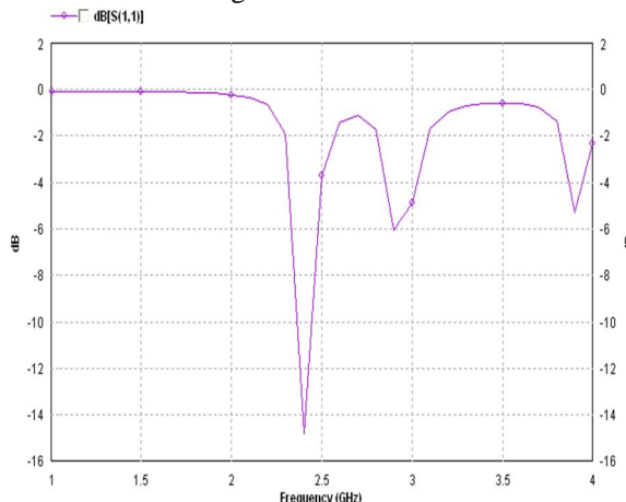
Figure 2(a): RL curve for the patch antenna
