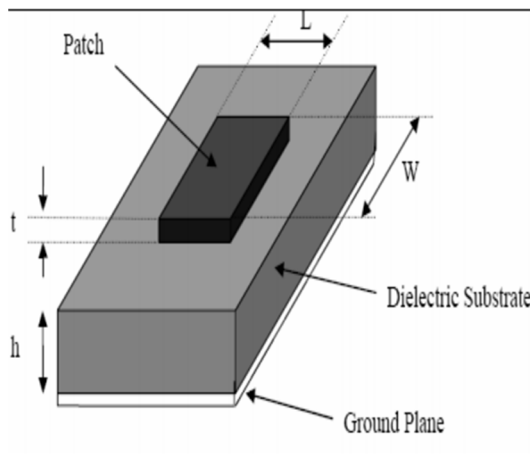
Figure 1: A Typical Microstrip Patch Antenna
