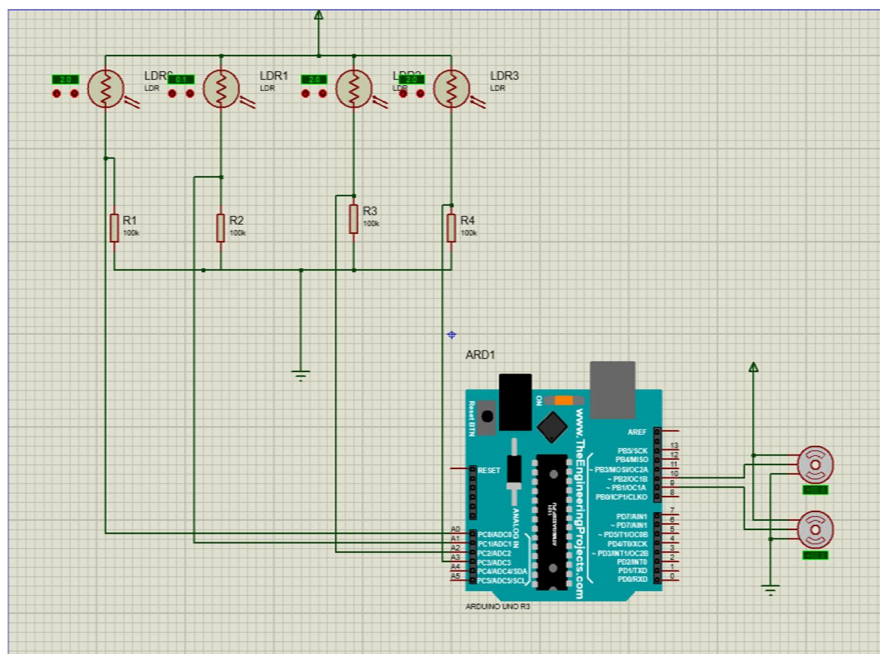
Fig3. Simulation circuit diagram of solar tracker
