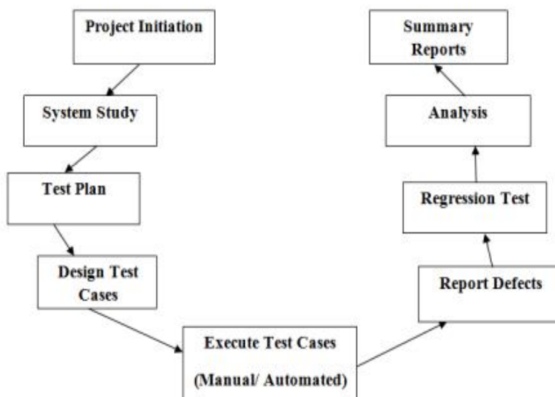
Fig. 2 Software Testing Life Cycle
