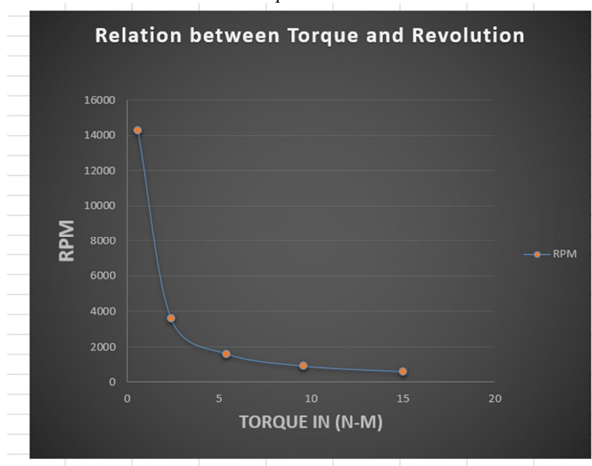
Torque Vs RPM
