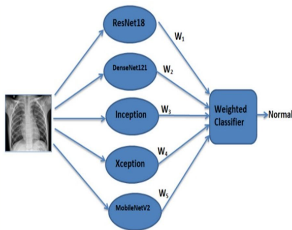
Figure 3. Weighted classifier module used in this paper (weighted predictions from all the models are passed to the weighted classifier, which gives the final weighted prediction).
