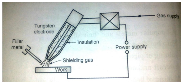
Fig No 13: Gas Tungsten Arc Welding
