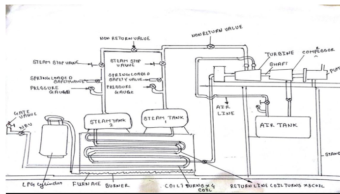
Diagram No 1: Construction & working of lifting water at remote places
