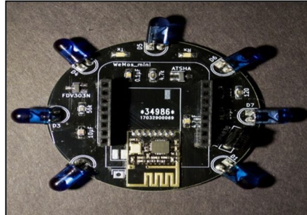
Figure 3 IR blaster 360
