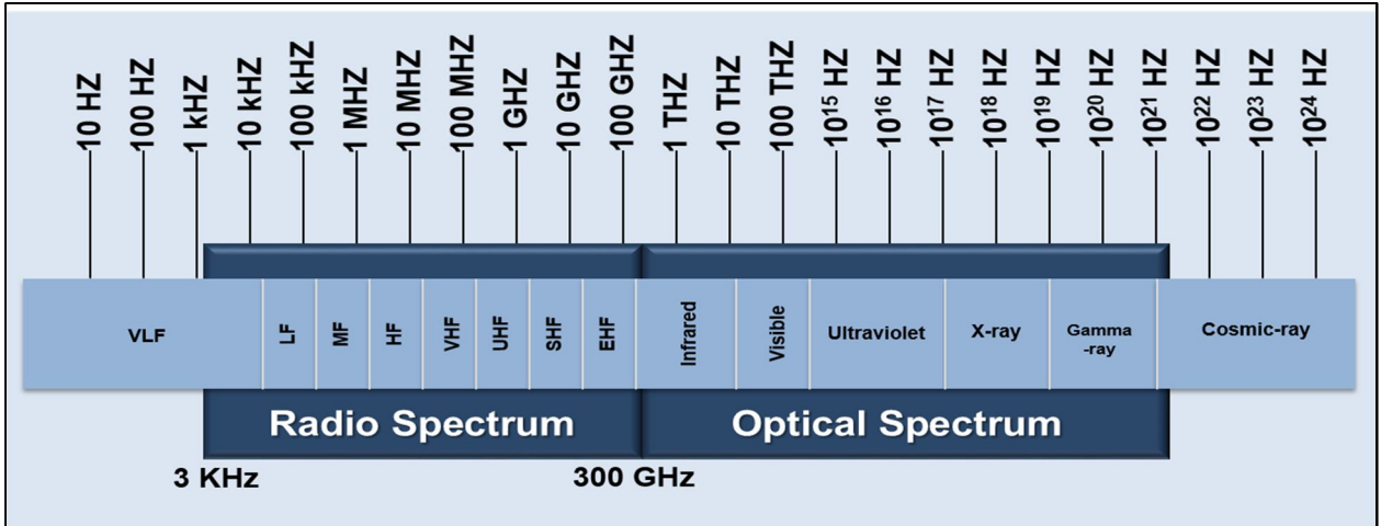
Figure 6 Electromagnetic Spectrum
