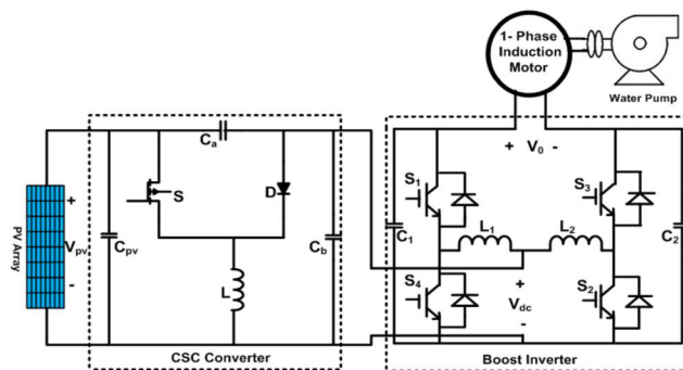
Fig. 1. CSC Converter fed Induction motor for Water pump
