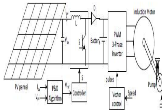
Fig.2.The suggested Induction motor photovoltaic pumping system configuration
