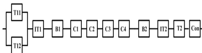
Figure 2. Reliability network diagram of the three-state UPFC model
