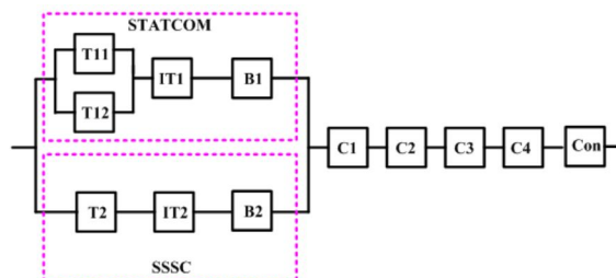
Figure 3. Reliability network diagram of a four-state UPFC model
