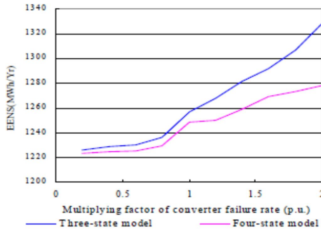
Figure 6. Impacts of converter failure rate on the EENS index
