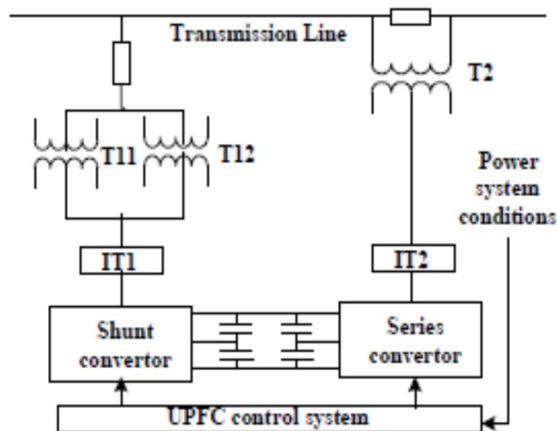
Figure 1. UPFC schematic diagram
