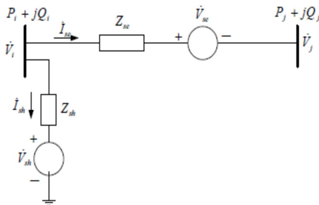
Figure 4. UPFC equivalent circuit
