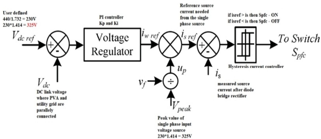
Fig 1.6 Block diagram of power flow converter control.
