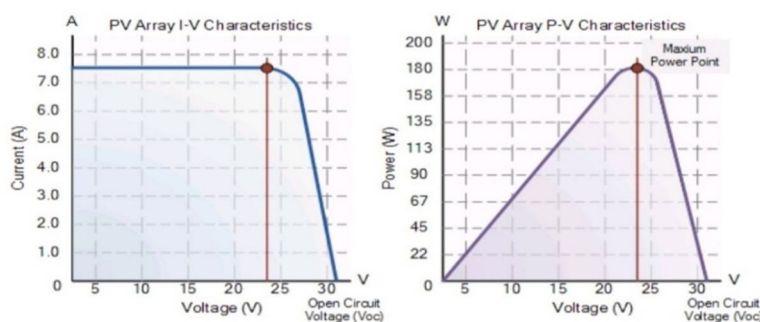
Fig 1.3 Characteristics of PV array.
