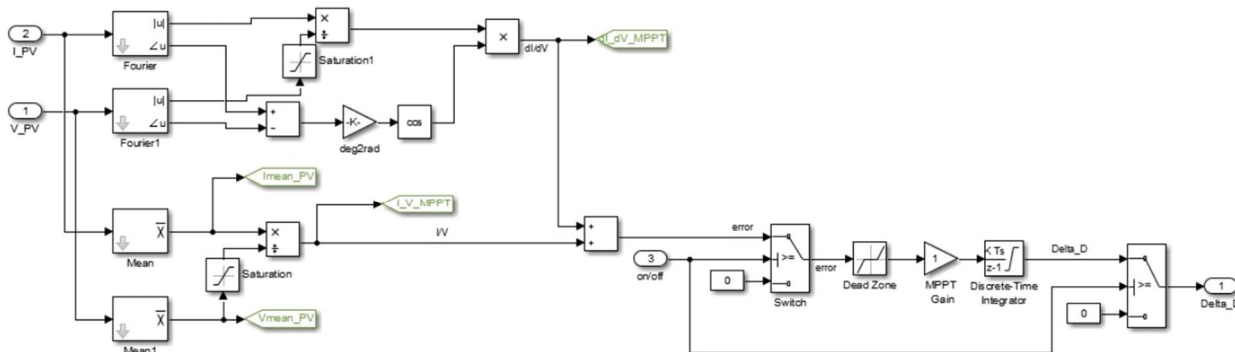
Fig 1.5 Modelling of incremental conductance MPPT method.
