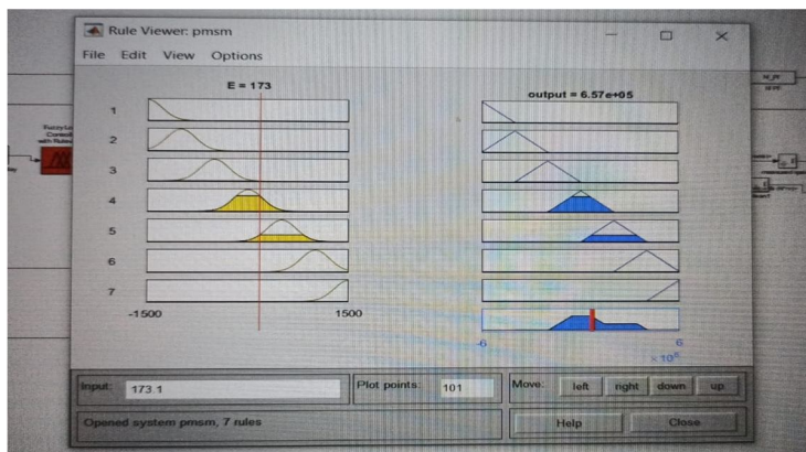
Fig 2.4 Rule viewer.
