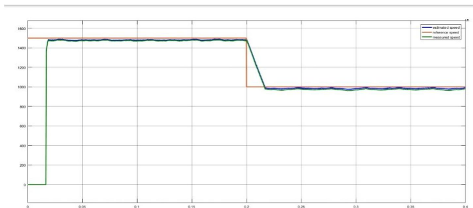
Fig 2.1 Speed of the machine compared with reference value.
