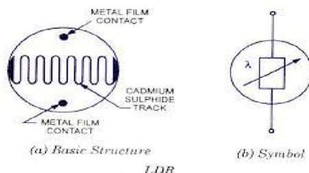
Figure.4: Light Dependent Resistor (LDR)
