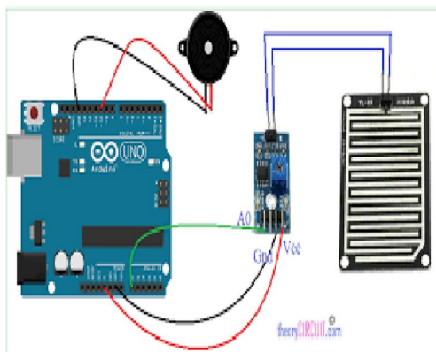
Figure .3: Arduino Rain sensor operational mechanism
