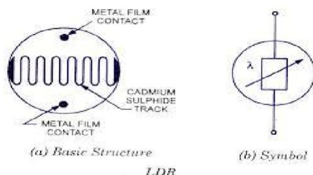
Figure.4: Light Dependent Resistor (LDR)
