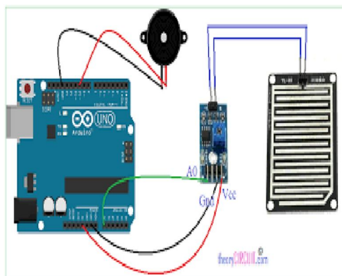
Figure .3: Arduino Rain sensor operational mechanism
