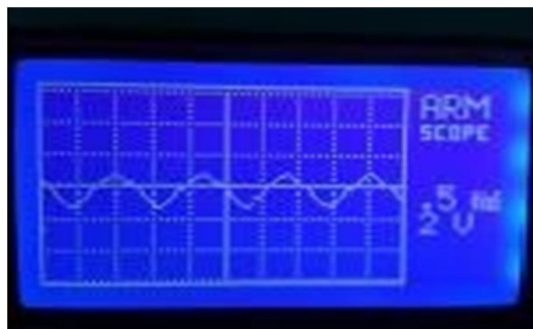
Figure 6.3: 2V and 1KHz Triangular Wave
