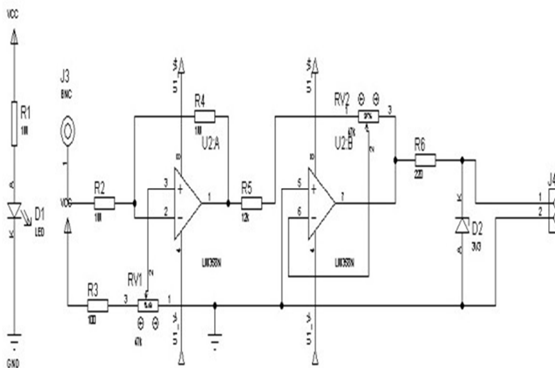
Figure 3.1: Comparator Circuit
