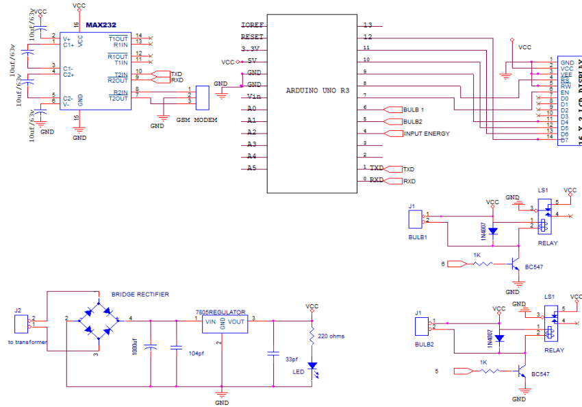
Fig.4.Schematic Diagram
