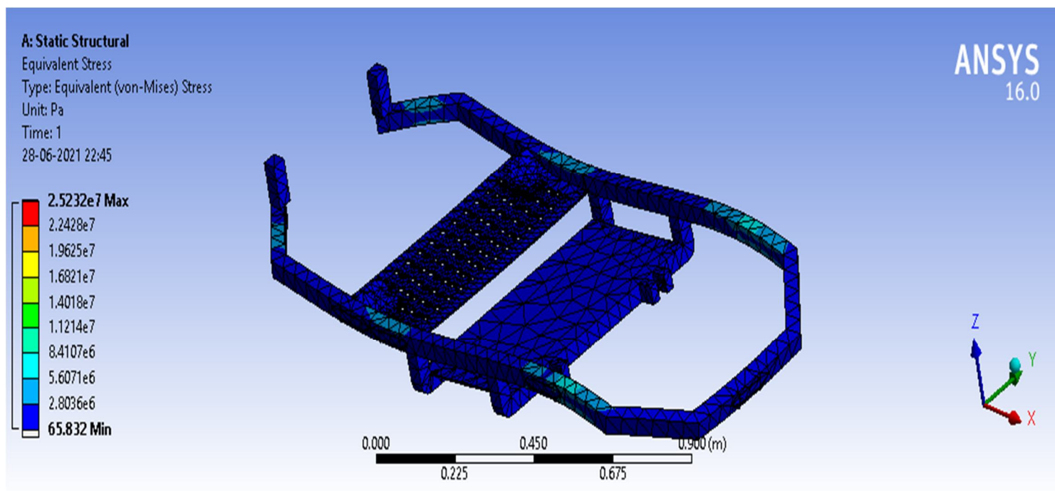
Fig. 2 analysis on chassis
