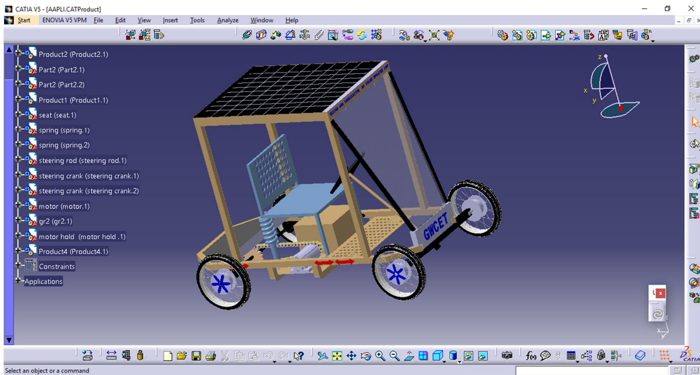
Fig. 1 cad model of a solar operated car
