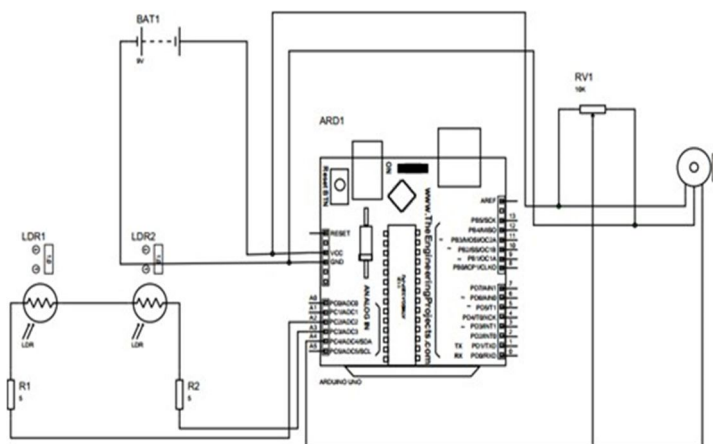
Figure 3: Schematic diagram of the solar panel tracking system.
