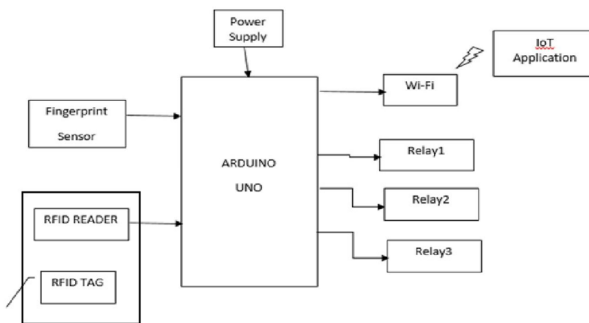
Figure 1: Block Diagram of the Lineman Safety
