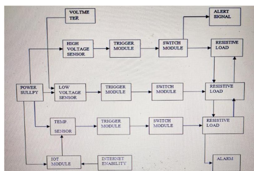
Fig 1 – Block Diagram
