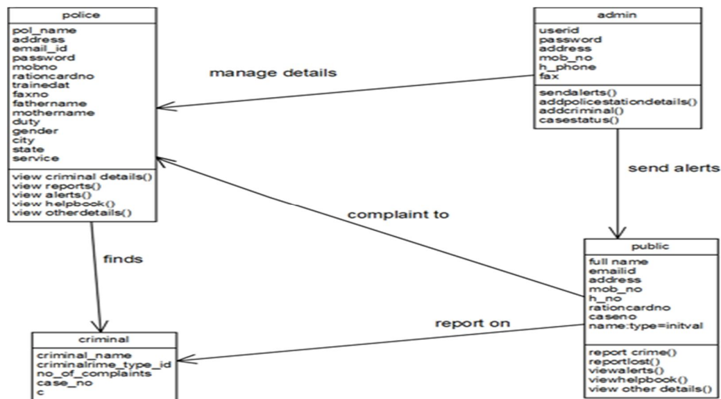
Fig. 2 Class Diagram
