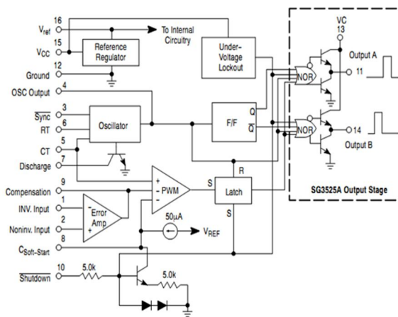
SG3525 Block Diagram
