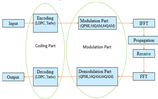
Fig.8. LDPC coded OFDM system
