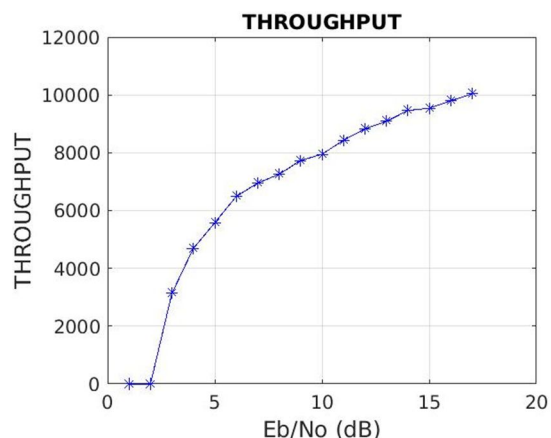
Fig. 10. Throughput vs SNR
