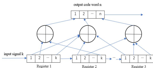
Fig.7. Convolutional Code
