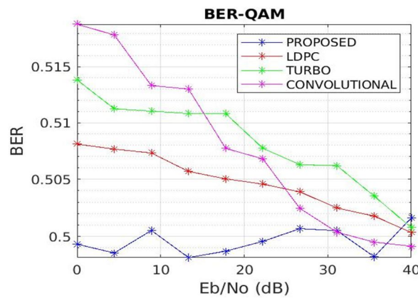
Fig. 8.b. Comparison of coding methods with QAM modulation
