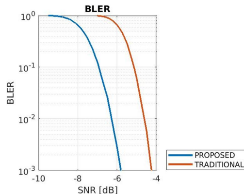
Fig. 9. BLER variation in the proposed system and traditional system
