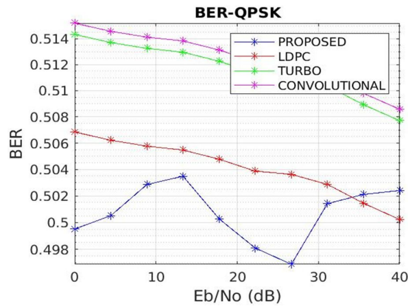
Fig. 8.a. Comparison of various Coding methods with QPSK modulation
