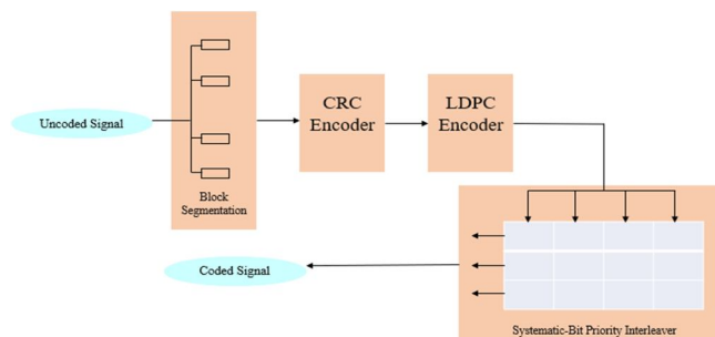
Fig. 6. LDPC Coding Process
