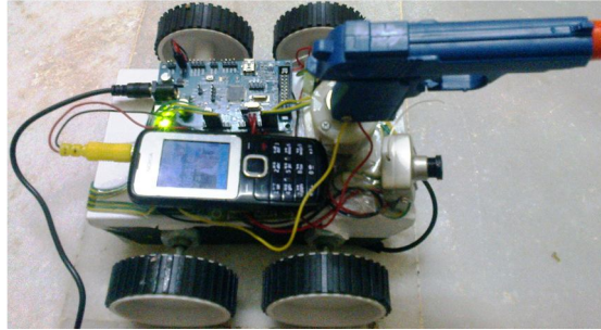
Fig.8: Implemented GSM controlled vehicle
