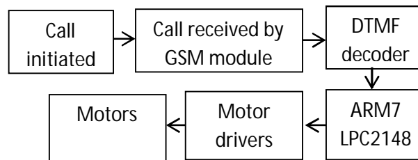
Fig.1: Block diagram of GSM based vehicle.
