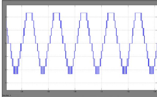
Fig.4.2. Output Current Waveform
