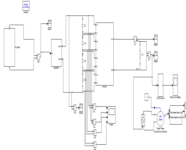
Fig 2 Simulation circuit for 9-level Cascaded Inverter
