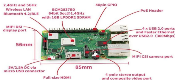
Fig. 2 Raspberry pi 3 B+
