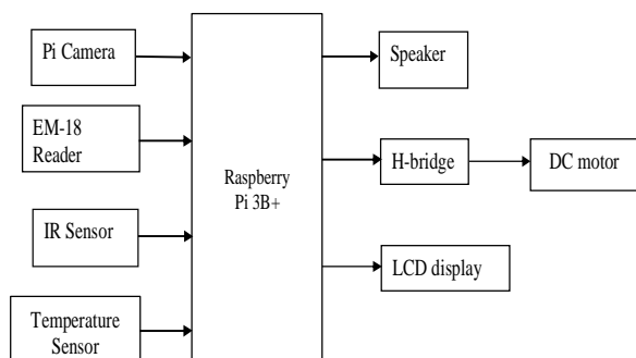
Fig. 1 Block diagram of Receptionist robot
