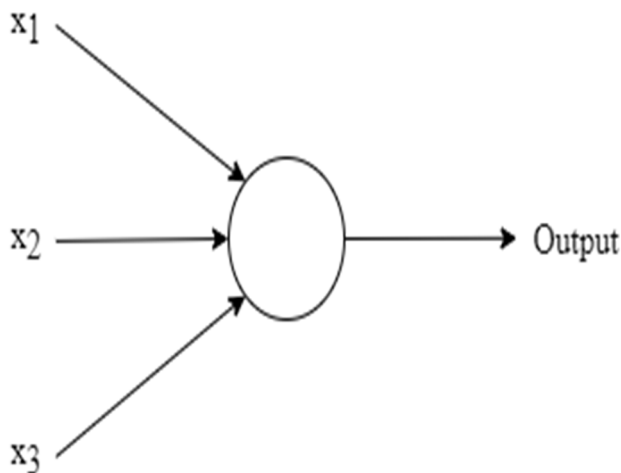
Figure 2: Perceptron
