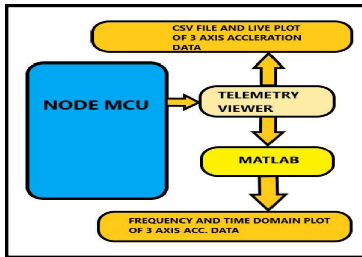
Fig.4.Telemetry and MATLAB connection diagram
