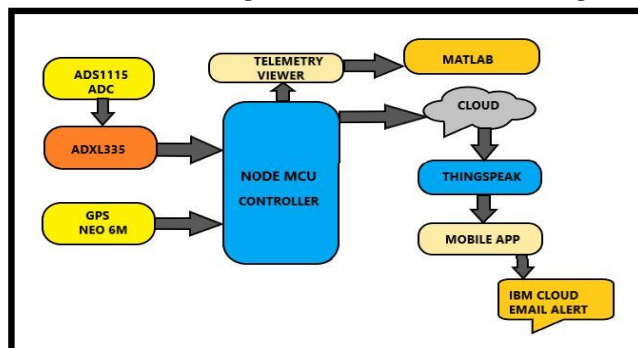
Fig. 2. System's Block diagram
