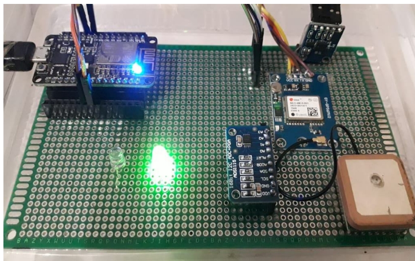
Fig.12. Working hardware of system
