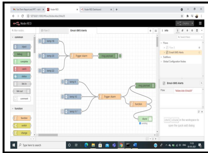
Fig.10. Node red mapping for alert system.
