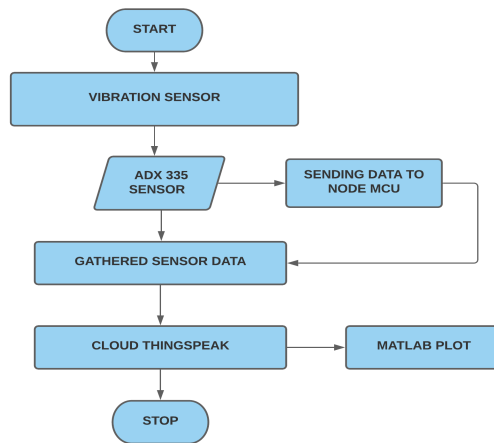
Fig. 1. System's flowchart
