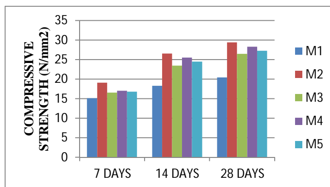
Fig. 1 : Compressive Strength Test Analysis
