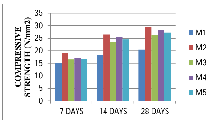
Fig. 1 : Compressive Strength Test Analysis
