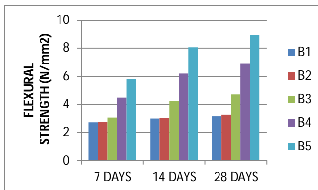
Fig. 2 : Flexural Strength Test Analysis
