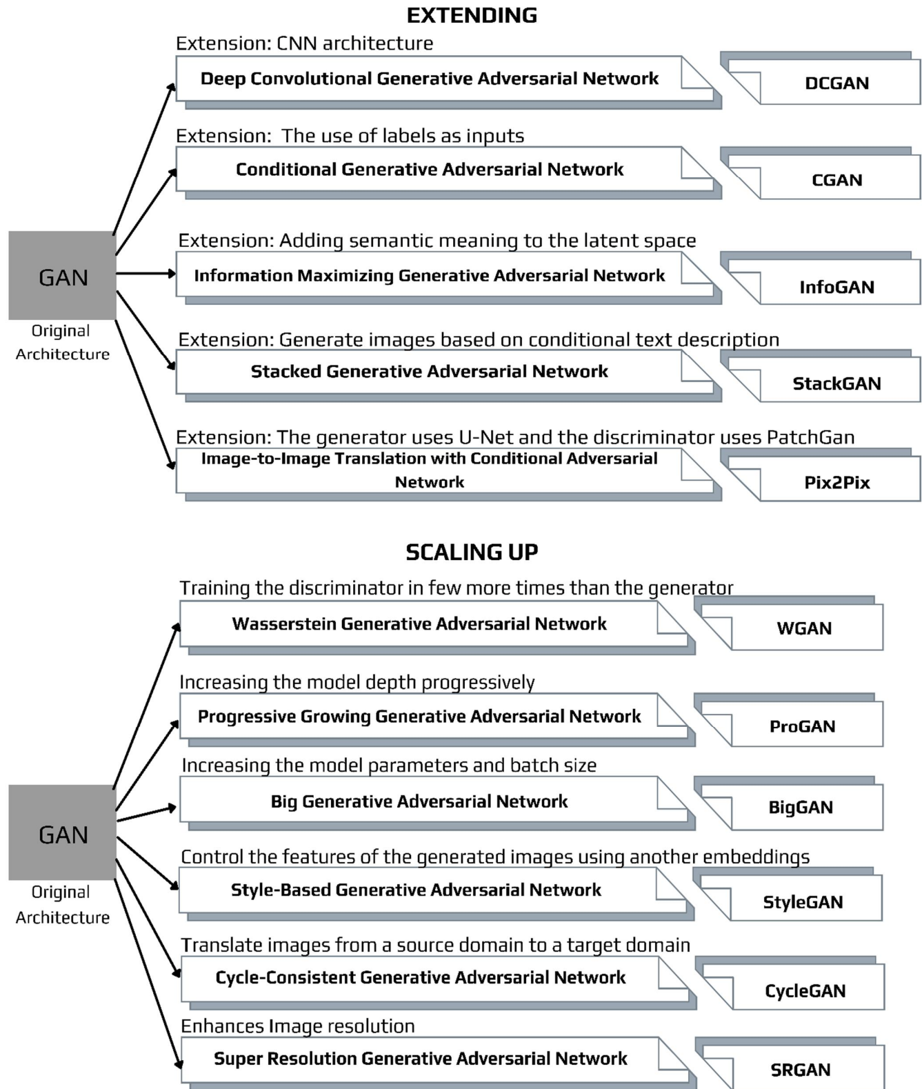
Figure 8: Types of GAN Model architectures and extensions
