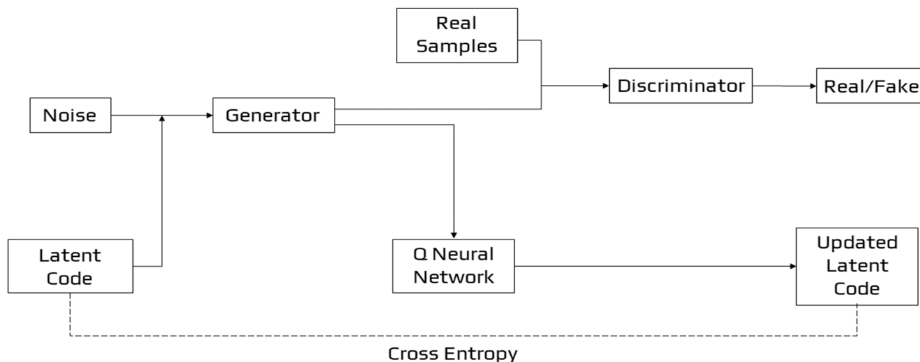
Figure 11: InfoGAN
