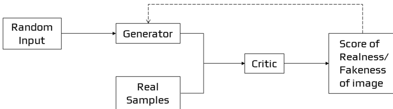
Figure 14: Wasserstein GAN
