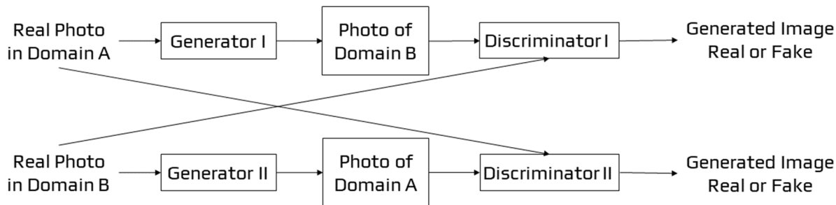
Figure 17: CycleGAN
