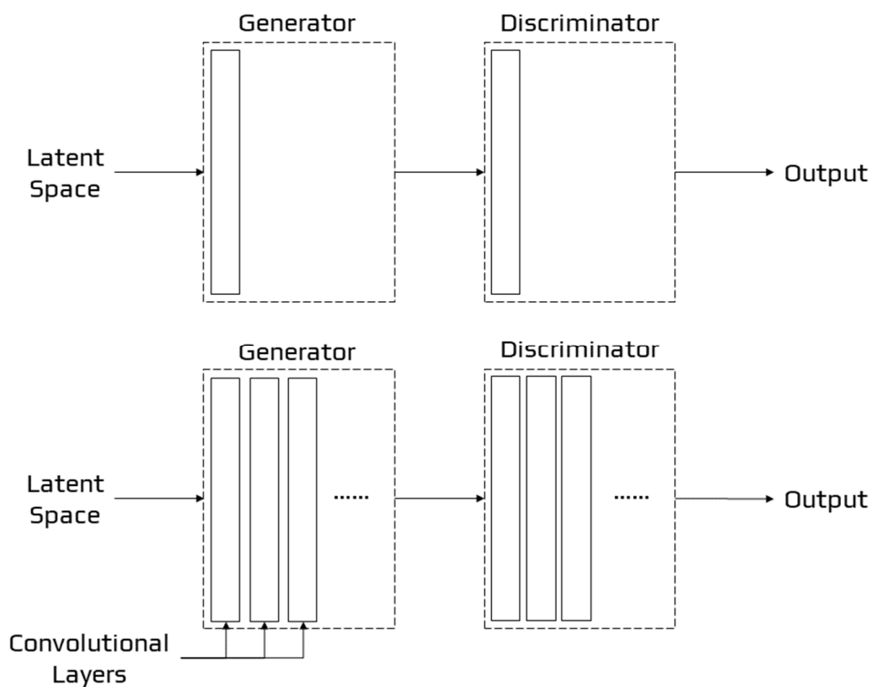
Figure 15: ProGAN
