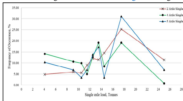
Fig. 12 Load Spectra for Single Axle
