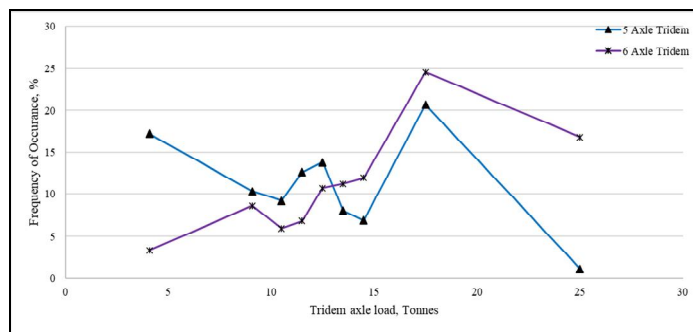
Fig. 14 Load Spectra for Tridem Axle
