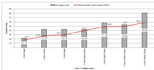
Fig. 10 Gross Vehicle Weight vs Permissible Load Limit
