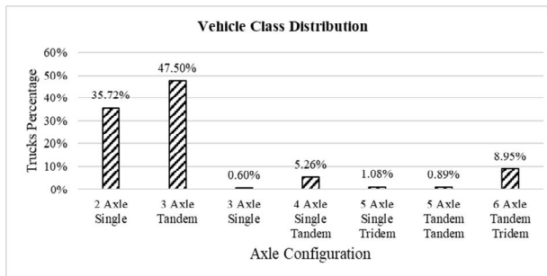
Fig. 8 Percent of trucks of different classes plying on National Highway
