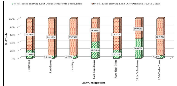
Fig. 11 Percent Trucks Carrying Load Under/Over Permissible Load Limit
