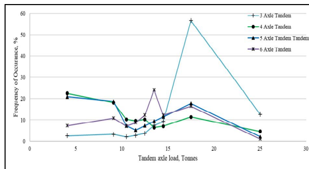
Fig. 13 Load Spectra for Tandem Axle
