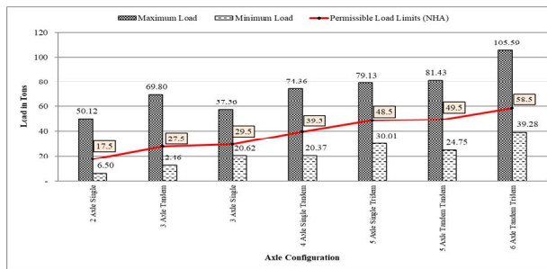
Fig. 9 Maximum, Minimum and Permissible Load Limit for Vehicle Classes
