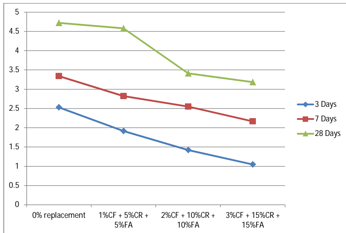
Graph (2) shows variations in Flexural strength
