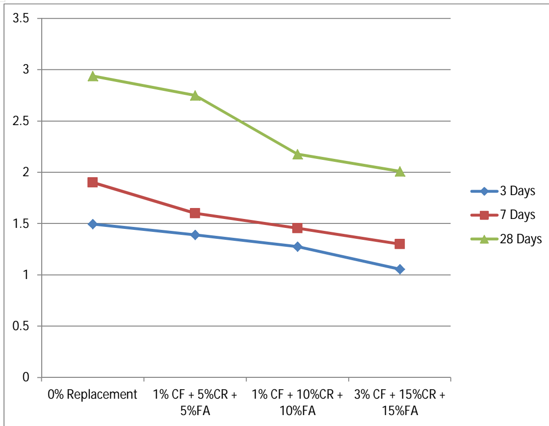
Graph (3) shows variations in Split tensile strength
