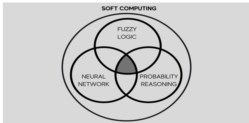
Figure 2: Soft Computing
