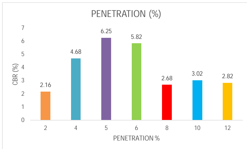
Figure. 6. CBR of clay soil with lime
