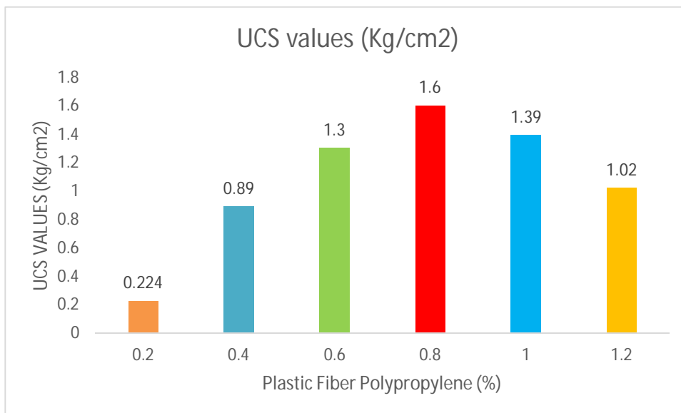
Figure. 7. UCS with varied plastic content
