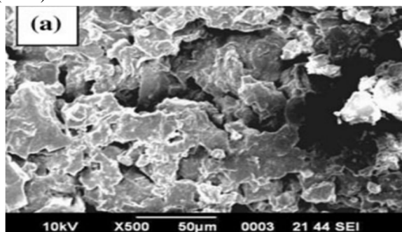
Figure 8. SEM images of soil
