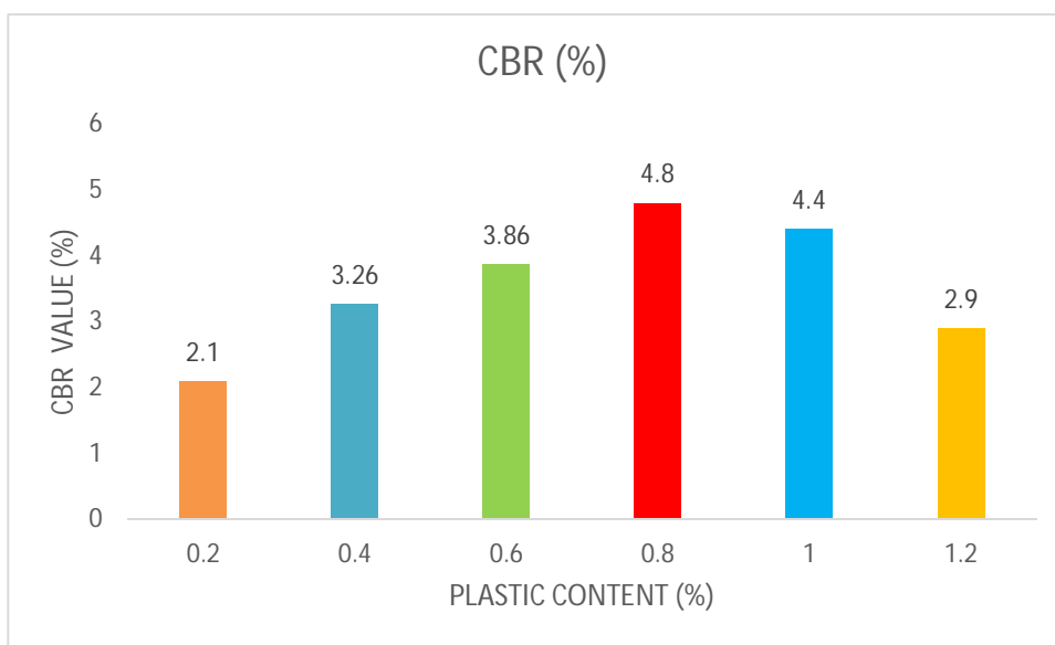
Figure. 5 CBR with different plastic content
