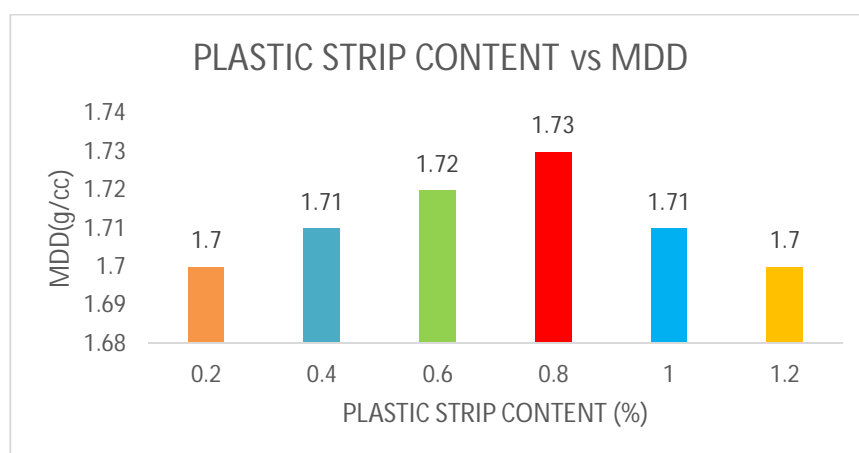
Figure 4. MDD w. r. t. Plastic Fiber
