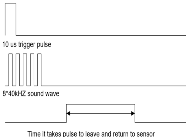
Fig. 3. Waveforms of Ultrasonic Sensor
