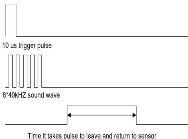
Fig. 3. Waveforms of Ultrasonic Sensor
