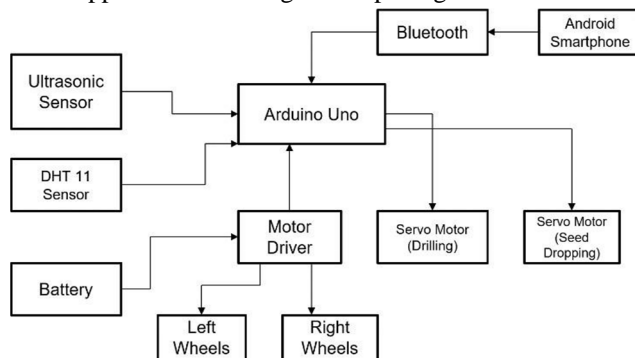
Fig. 5. Block Diagram of Seed Sowing Robot
