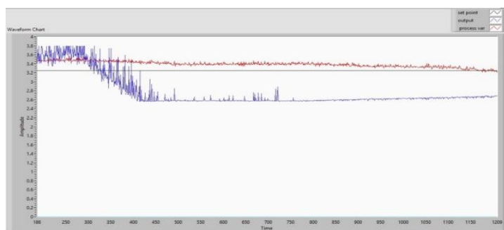
Fig.5 Fuzzy logic controller with 5% concentration of nanofluid
