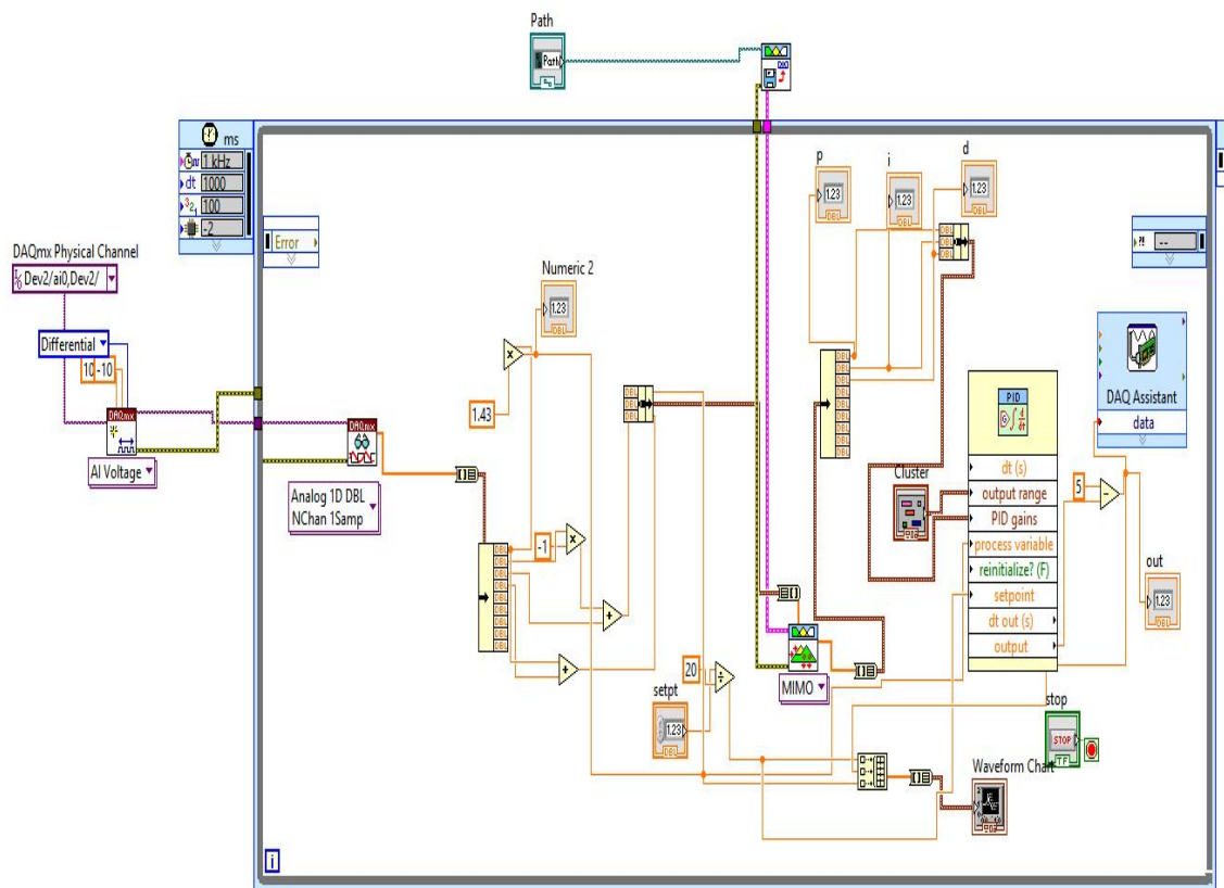
Fig.2 Graphical representation of software program
