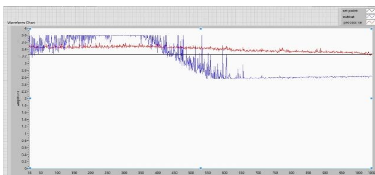
Fig.6 Hybrid controller with 5% concentration of nanofluid
