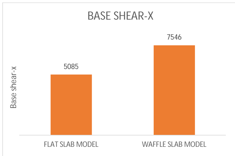
Figure 8: Graphical representation Base shear X
