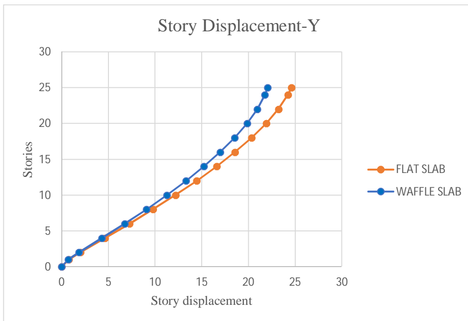
Figure 5: Represents comparison of story displacement in y direction
