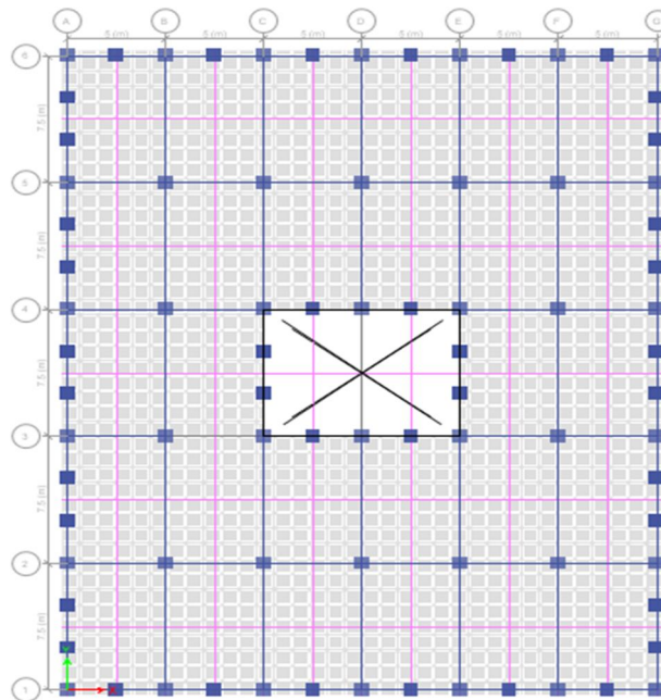
Figure 3: Plan view of structure with waffle slab
