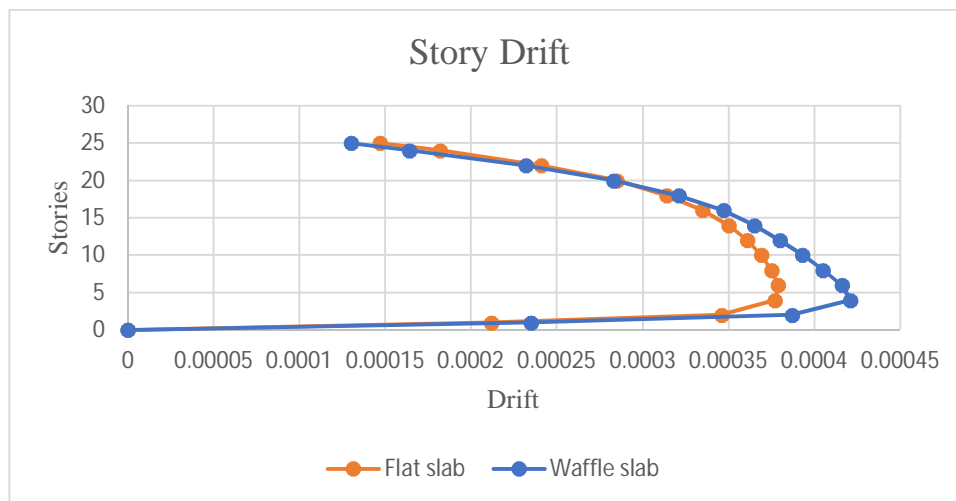
Figure 6: Represents comparison of story drift in x direction
