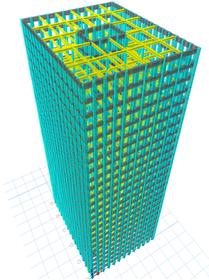
Figure 1:3D view of tube in tube structure
