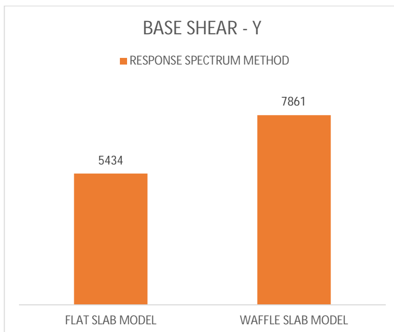
Figure 9: Graphical representation Base shear Y
