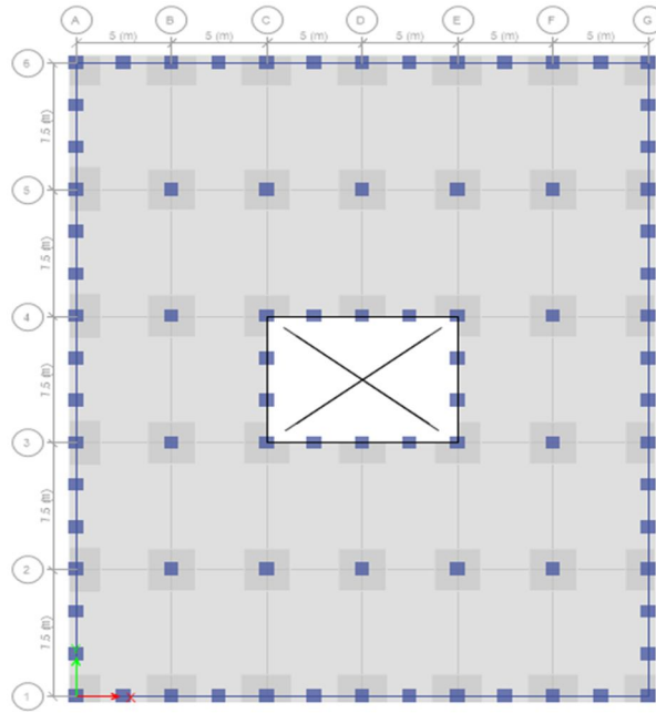
Figure 2: Plan view of structure with flat slab
