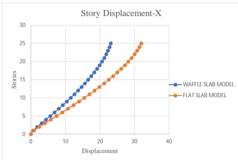
Figure 4: Represents comparison of story displacement in x direction
