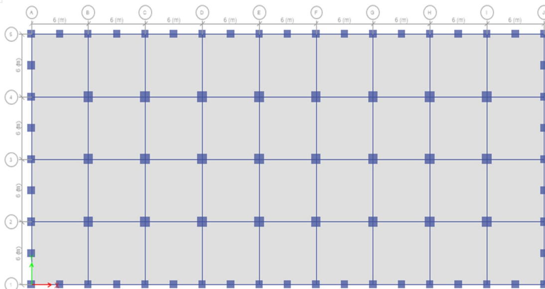
Figure 3: Plan view of RC normal frame
