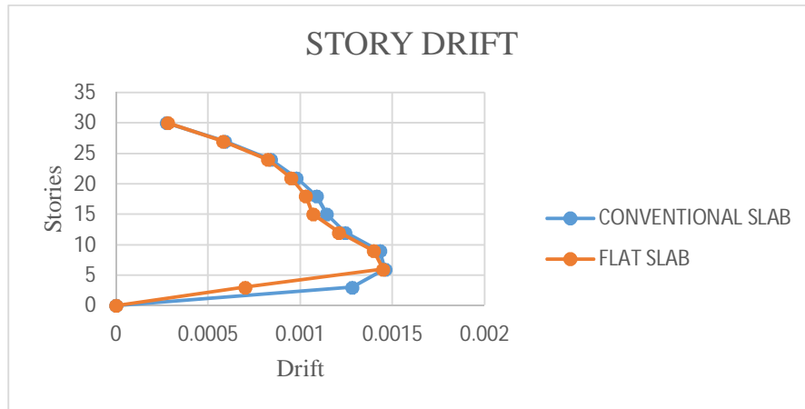
Figure 10: Represents comparison of story drift between conventional slab with framed tube system and flat slab with framed tube system.
