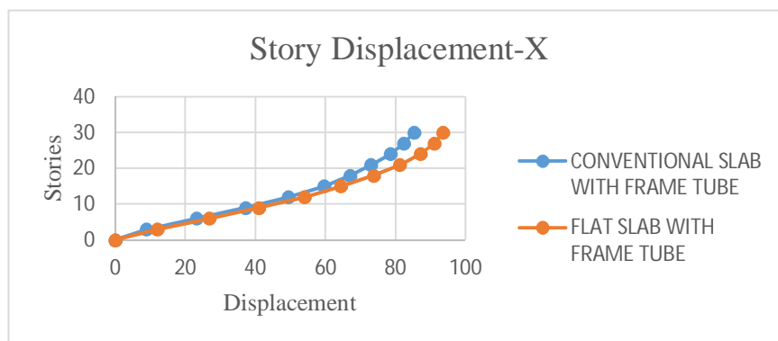
Figure 5: Represents comparison of storey displacement between conventional slab and flat slab with framed tube system in X-direction.
