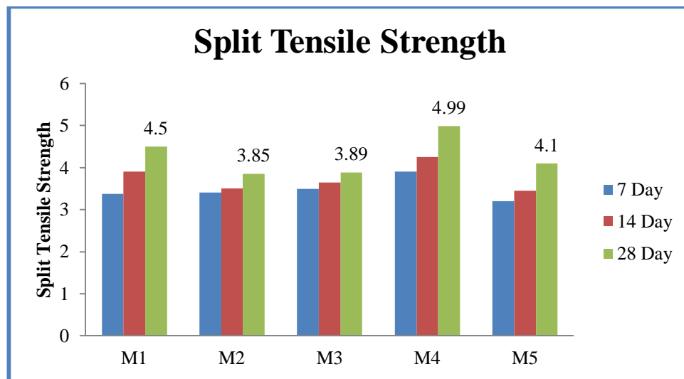
Fig. 4.2 Variation of split tensile strength of concrete with age
