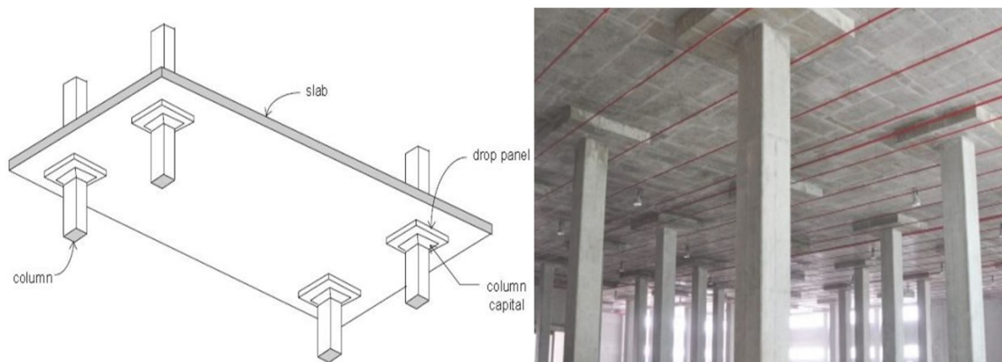
Fig. 3: Typical examples of flat slab
