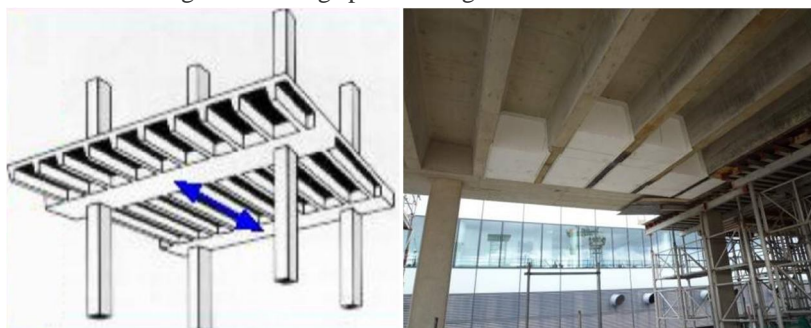
Fig. 2: Typical examples of ribbed slab
