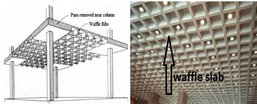
Fig. 1: Typical examples of waffle slab
