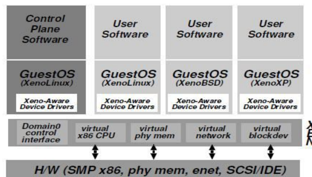
Fig. 6 The Structure of machine running the Xen Hypervisors
