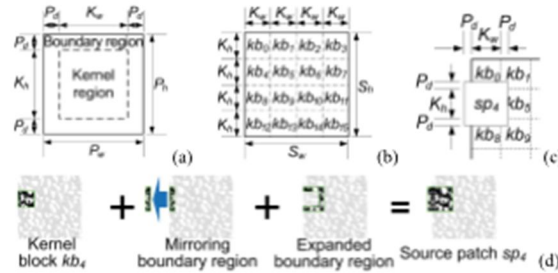
Fig. 1. Patch, kernel blocks, and source patch.
