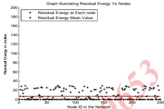
Fig 13: Nodes energy residue in first level hierarchical technique for three cluster after 400 round simulation
