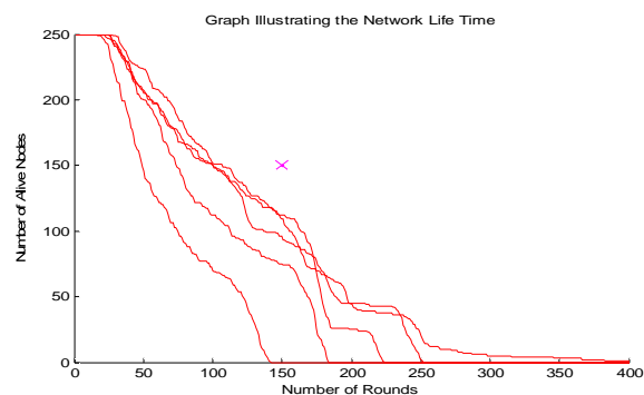
Fig 10 : Network lifetime graph (number of alive nodes for a particular round of simulation) in non-hierarchical, one level & two level hierarchical technique
