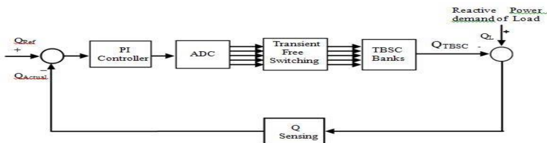
Fig.2 TBSC Closed loop operation.
