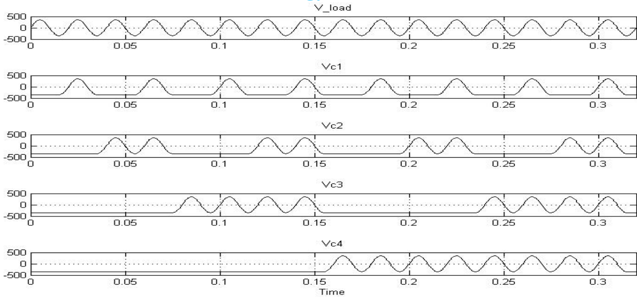
Fig.4 Voltage across capacitor (Vc1, Vc2, Vc3, Vc4).
