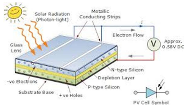
Fig. 1 Principle of PV Cell
