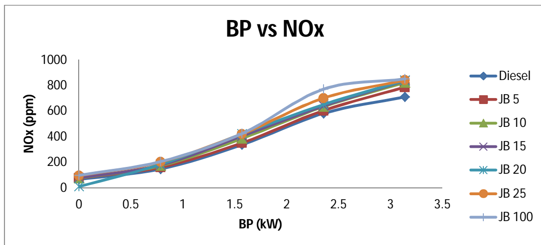
Fig-6 Effect of Engine Brake Power on NO x Emissions
