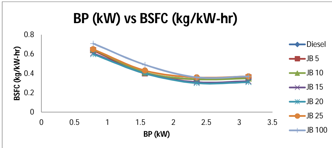
Fig-3 Effect of Engine Brake Power on Brake Specific Fuel Consumption
