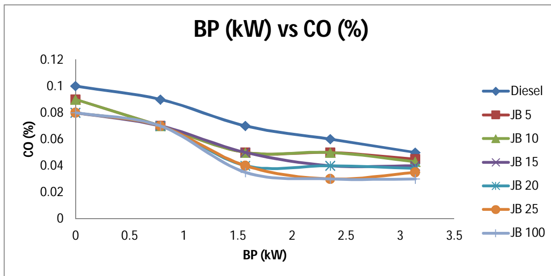
Fig-4 Effect of Engine Brake Power on CO Emissions
