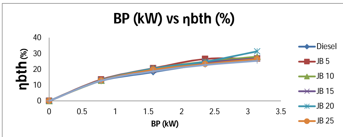
Fig-2 Effect of Engine Brake Power on Brake Thermal Efficiency
