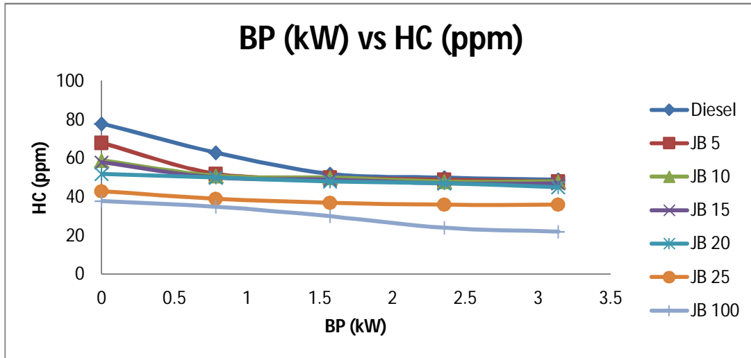
Fig-5 Effect of Engine Brake Power on HC Emissions
