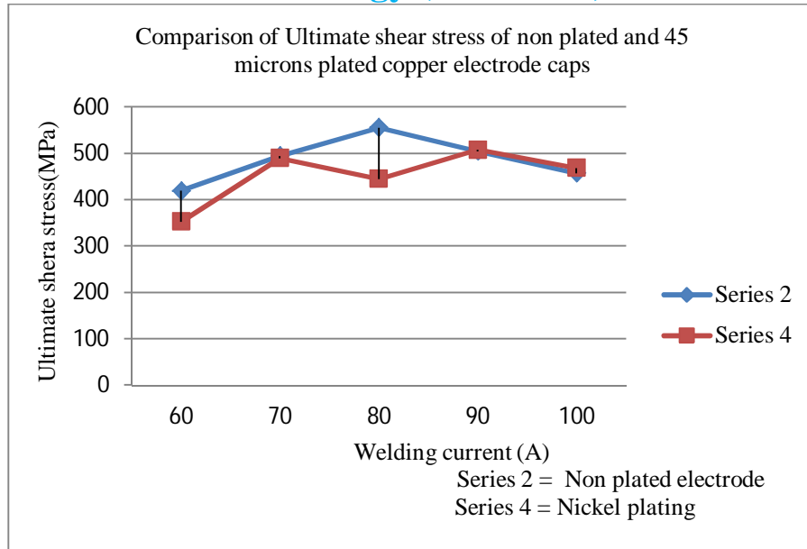
Fig 11: Effect of welding current and 45 microns plating on maximum load carrying capacity.
