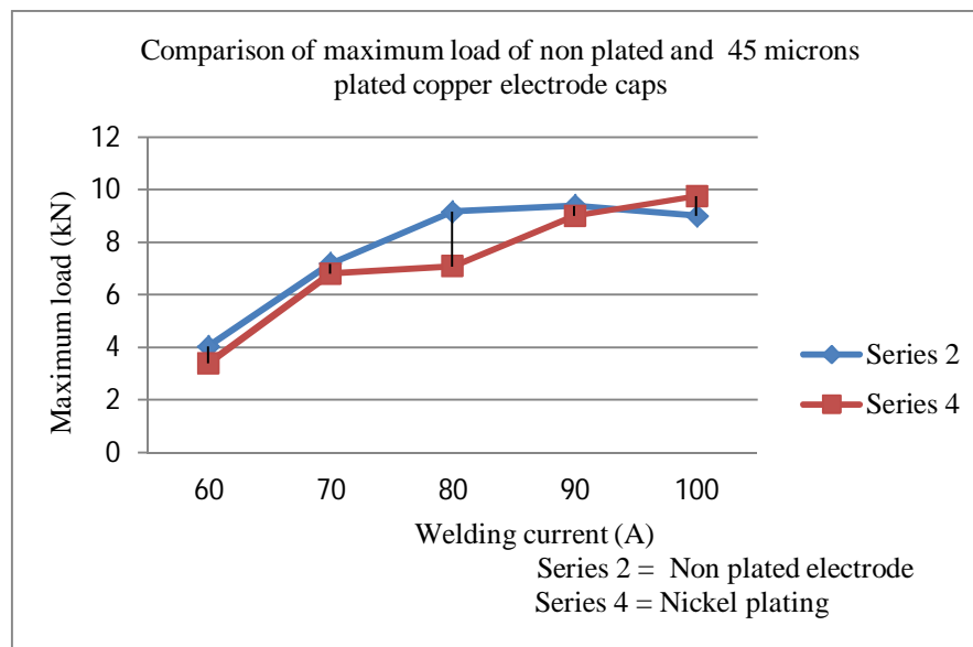
Fig 10: Effect of welding current and 45 microns plating on maximum load carrying capacity.
