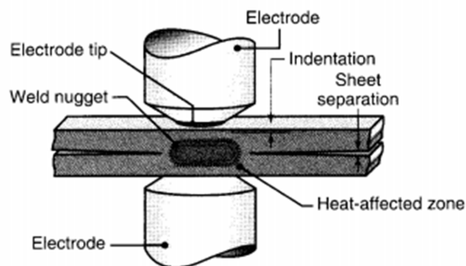
Fig 1: Cross section of a spot weld, showing the weld nugget and the indentation of the electrode on the sheet surfaces. The magnitude of the current, the resistance of the current conducting path, and the time for which the current is made to flow account for the heat generated in the workpiece. This can be expressed in terms of Joule heating, by the simple application of Ohm's law the voltage ( V ) required for a current flow ( I ) is given by the relationship
