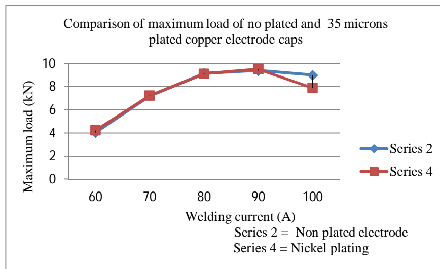
Fig 8: Effect of welding current and 35 microns plating on maximum load carrying capacity.
