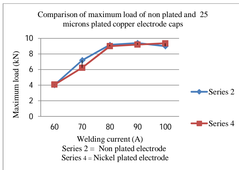
Fig 6: Effect of welding current and 25 microns plating on maximum load carrying capacity.
