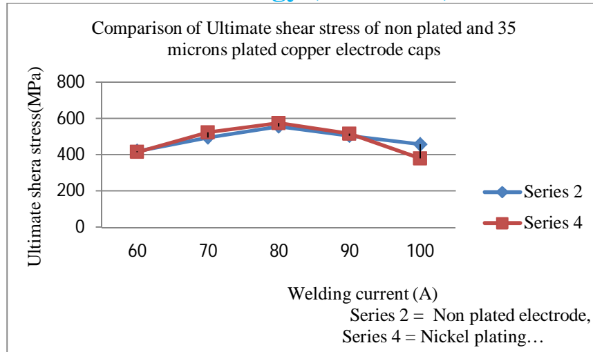
Fig 9: Effect of welding current and 35 microns plating on ultimate shear strength.
