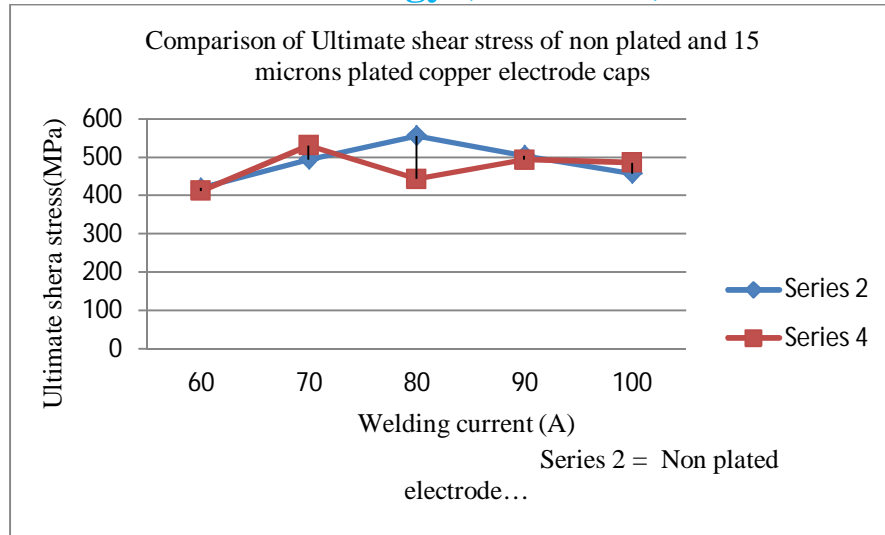
Fig 5: Effect of welding current and 15 microns plating on ultimate shear strength.
