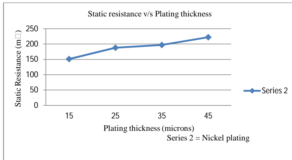
Fig 3: Effect of plating thickness on static resistance of the weld system.
