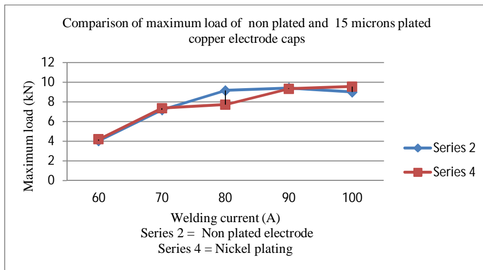
Fig 4: Effect of welding current and 15 microns plating on maximum load carrying capacity.
