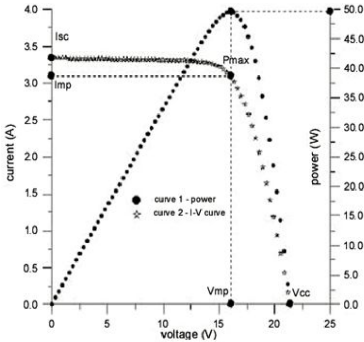
Fig:2 VI and PV characteristics of solar cell
