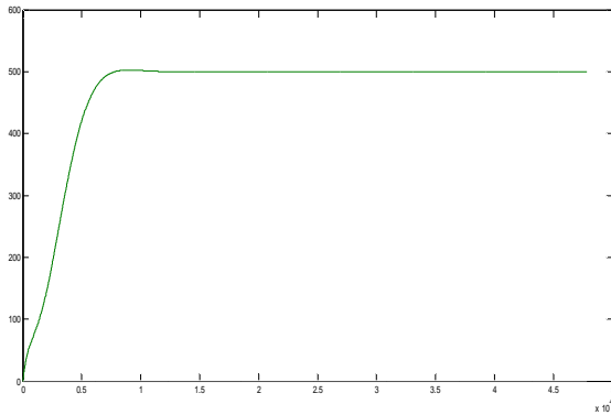
Fig: 9 Output Power of PV source (Cuk converter)
